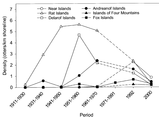
FIG. 2.—Temporal changes in density of sea otters for major island groups, 1911–2000. Representative densities for each period were based on maximal counts by aircraft for each island divided by the length of shoreline surveyed for each group. Dashed lines indicate when no data were available.
