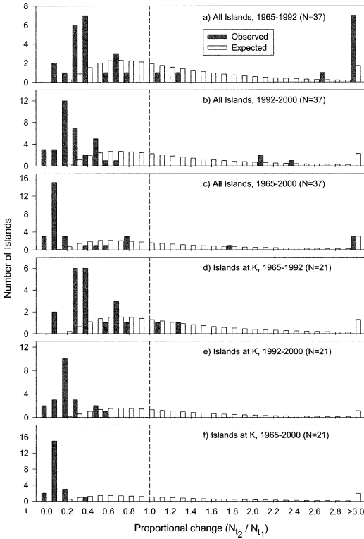
FIG. 3.—Frequency distributions of proportional changes in abundance ( N_{12}/N_{11} ) of sea otters among islands in the Aleutian archipelago. a–c) All islands surveyed during both years for which \geq 20 otters were counted during at least 1 survey and d–f) only for those islands which were at or near K (defined as the population status when growth ceased because of resource limitation) in 1965.
