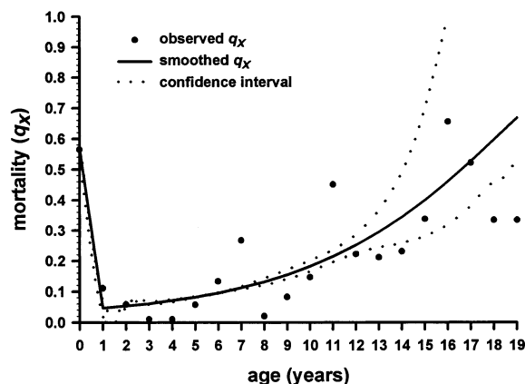
Fig. 7. q_x curve for sea otters at Amchitka Island, Alaska, based on the age distribution of beach-cast carcasses. Survival to age 1 estimated from the weaning success of pups born to radio-instrumented adult females. q_x curve computed as non-linear regression fit to mean values for each age-class (closed circles).
